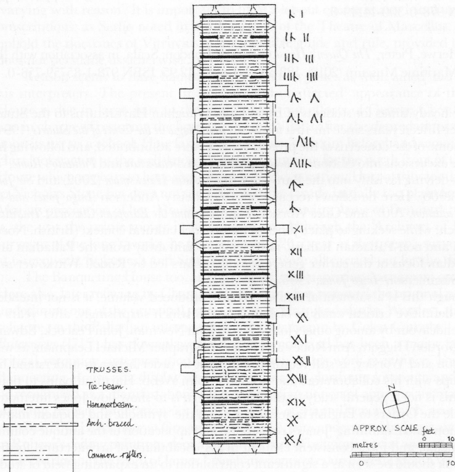
Paston (Norfolk), revised plan of the barn with the roof trusses numbered from north to south.
